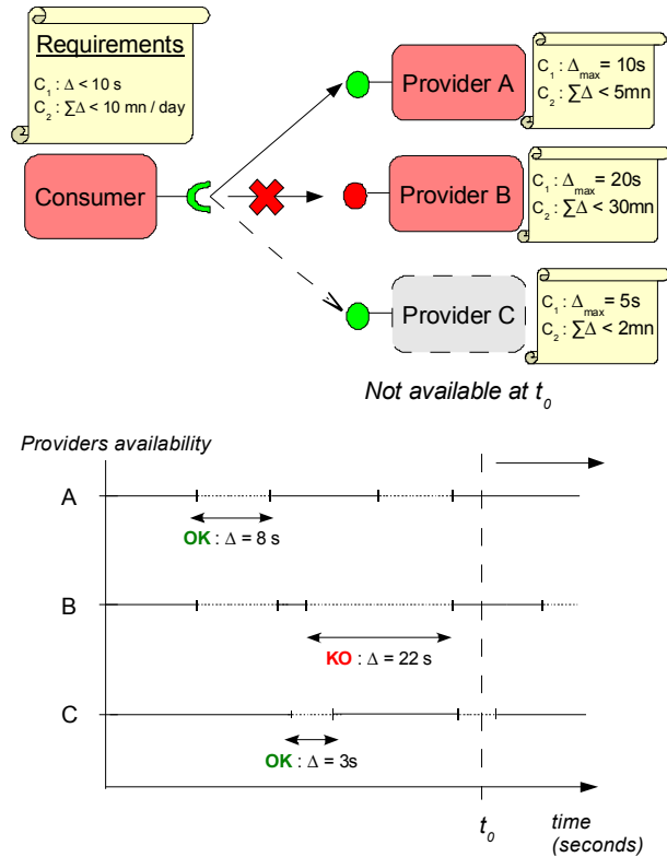
Figure 2. Service selection according to service disruption criteria and historical providers' availability
