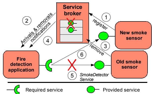
Figure 1. Service substitution scenario
